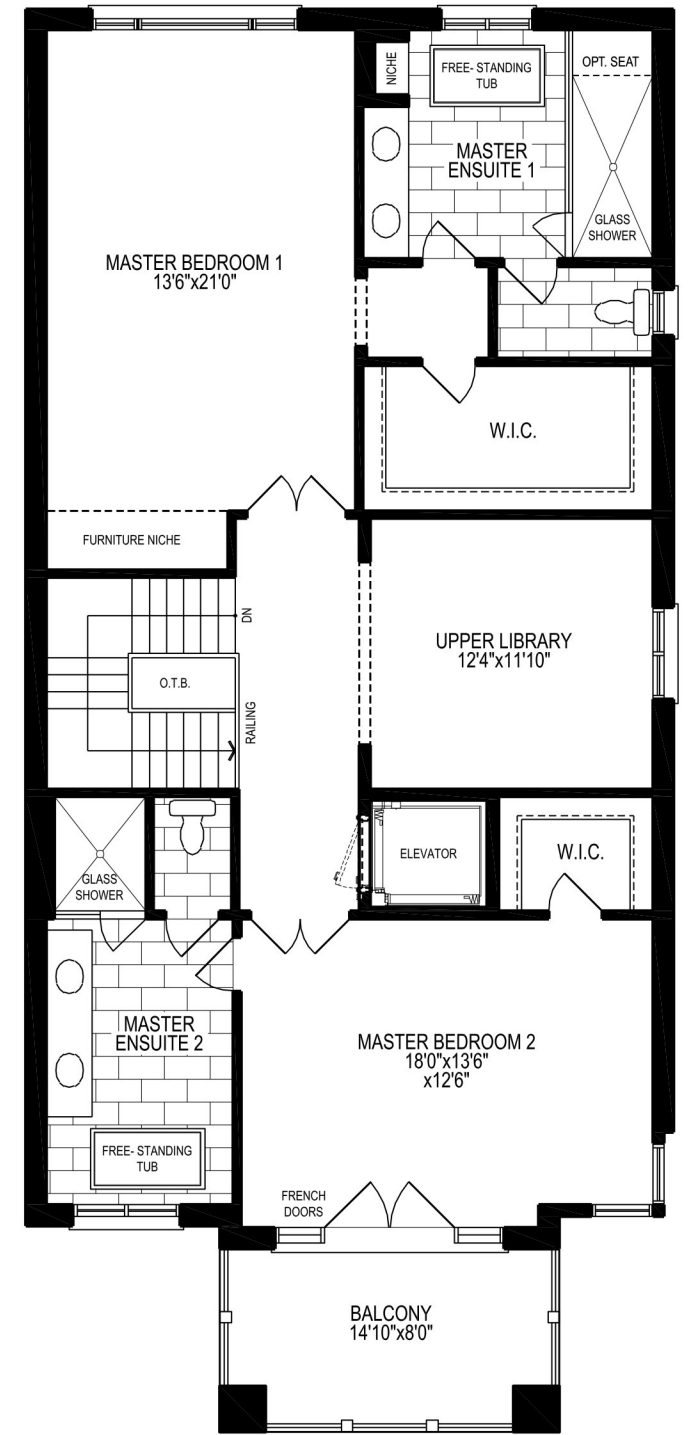
OPT. THIRD FLOOR PLAN, ELEV. 'A'
