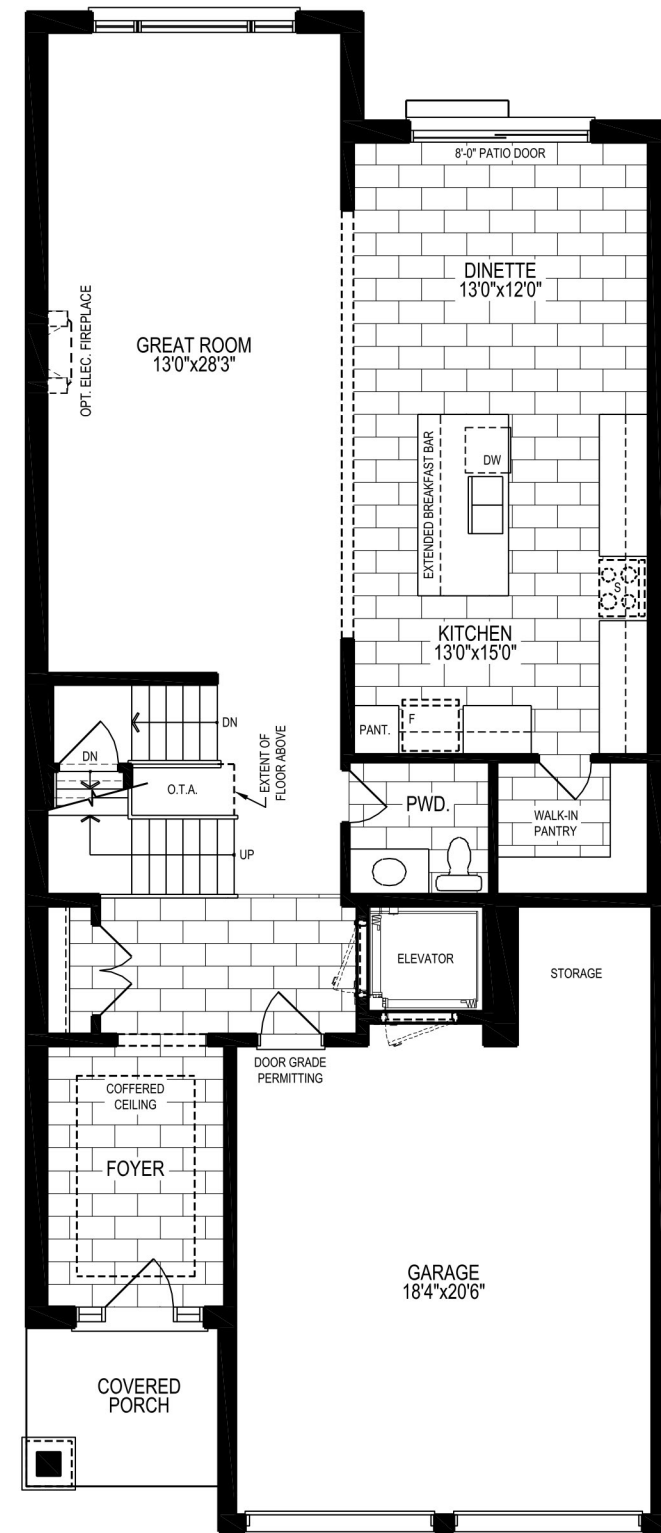
ALT. GROUND FLOOR PLAN, ELEV. 'A'
