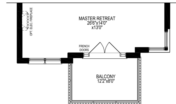
PART. THIRD FLOOR PLAN, ELEV. 'B'
