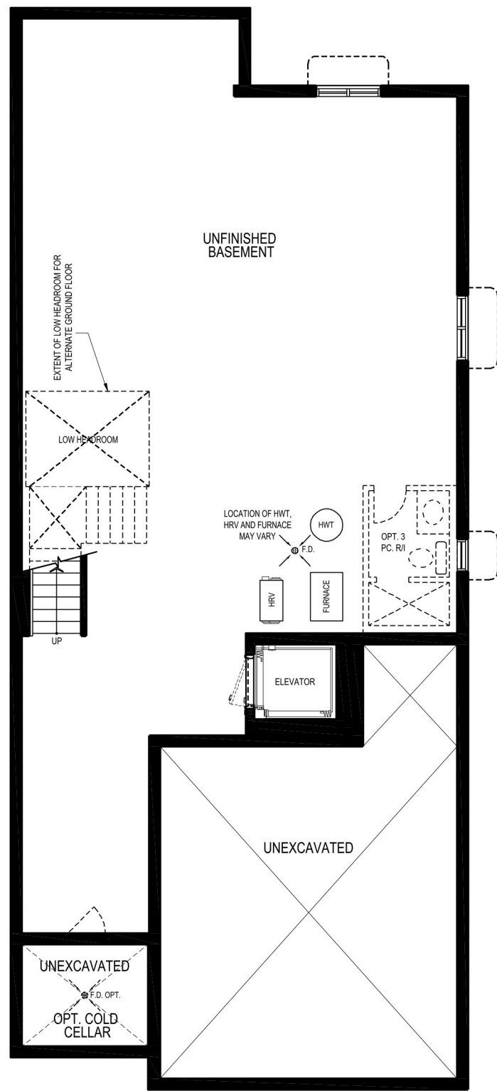
BASEMENT PLAN, ELEV. 'A'
