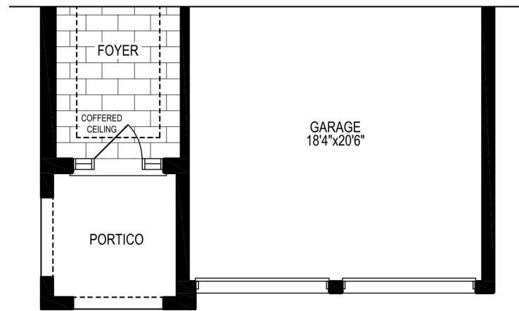
PART. GROUND FLOOR PLAN, ELEV. 'B'
