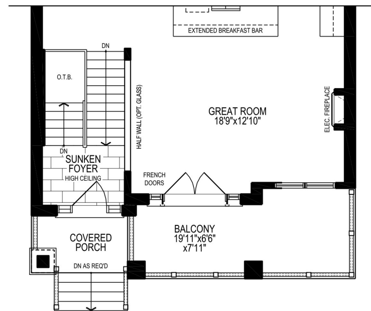
PART. OPT. MAIN FLOOR PLAN (2ND FLOOR) ELEV. 'B', W/ GREAT ROOM AT FRONT
