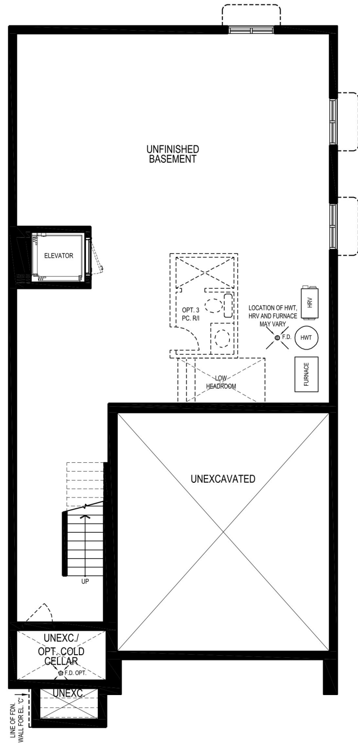
BASEMENT PLAN, ELEV. 'A', 'B' & 'C'
