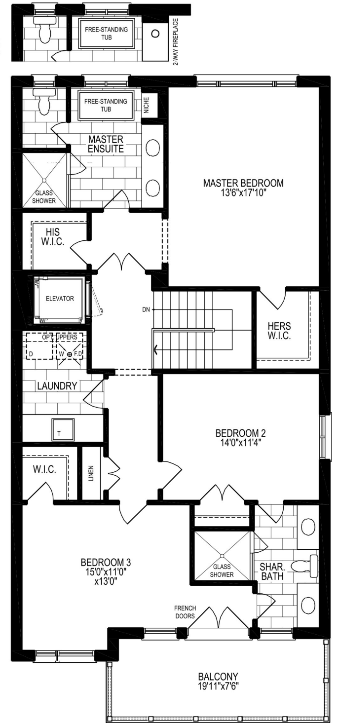
THIRD FLOOR PLAN, ELEV. 'A'
