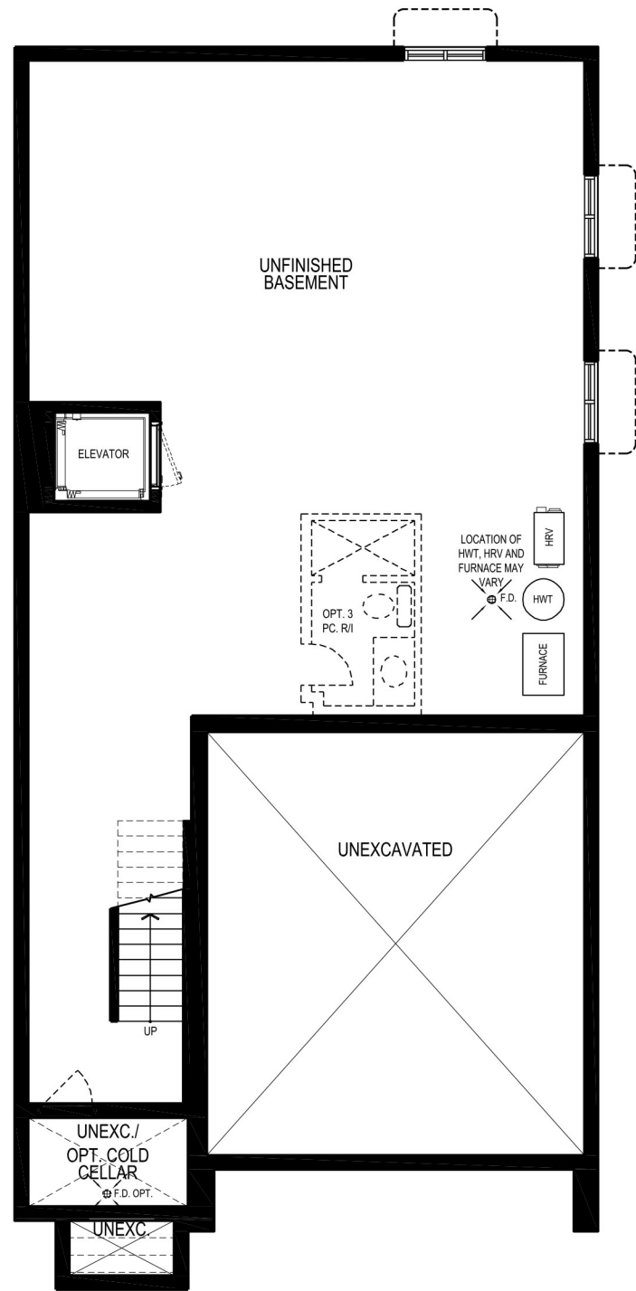
OPT. BASEMENT PLAN, EL. 'A', 'B' & 'C'
