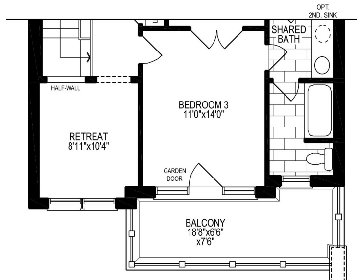
PART. SECOND FLOOR PLAN, ELEV. 'B'
