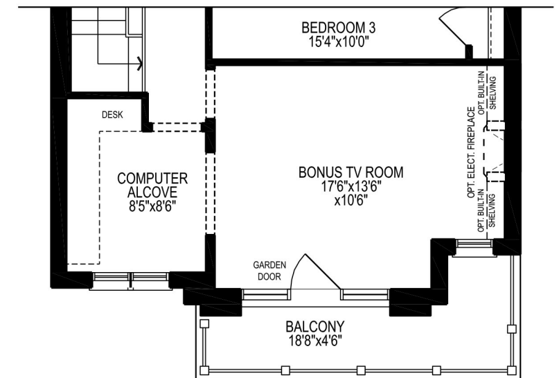
PART. ALT. OPT. SECOND FLOOR PLAN, ELEV. 'C', W/ ELEVATOR & BONUS TV ROOM
