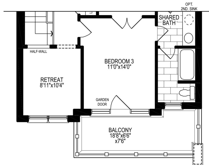
PART. OPT. SECOND FLOOR PLAN, ELEV. 'B', W/ ELEVATOR
