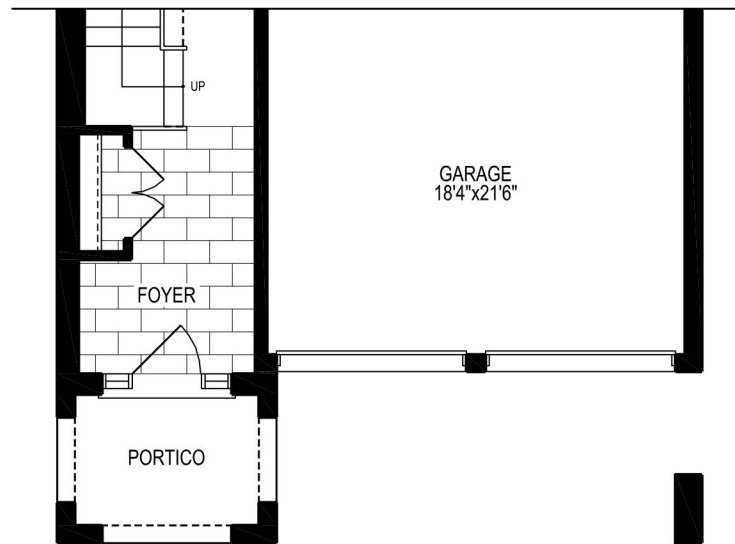
PART. GROUND FLOOR PLAN, ELEV. 'B' (OPT. ELEVATOR PLAN SIMILAR)
