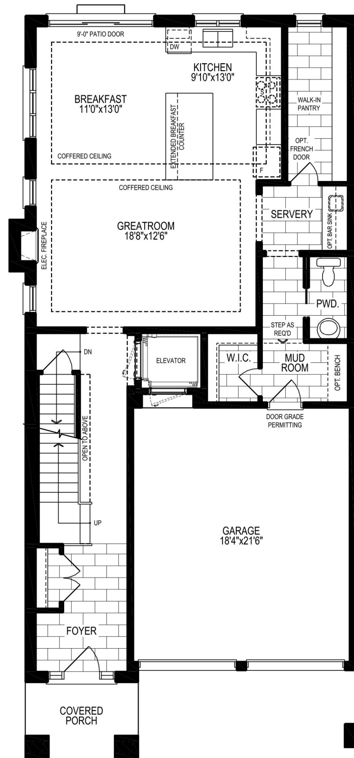
ALT. OPT. GROUND FLOOR PLAN, ELEV. 'A', W/ ELEVATOR (EL. 'B' & 'C' SIMILAR)
